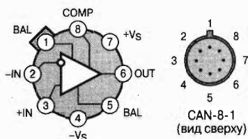
К140УД16, 140УД7/701, К140УД7/701
